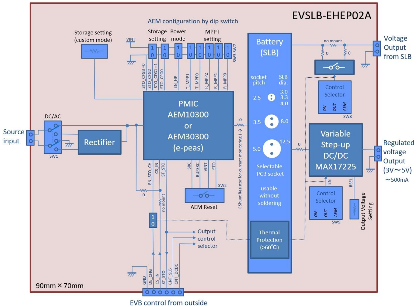
Fig 3 Block diagram
