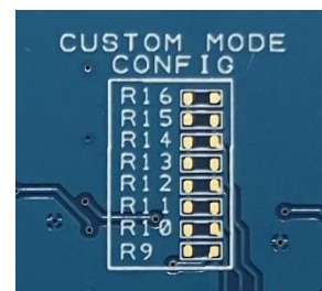
Fig. 4-3-1a Resistor lands for custom mode configuration
